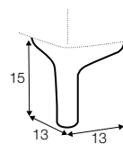
no. 218 wood
