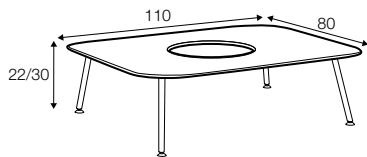
coffee table 1B 110x80
