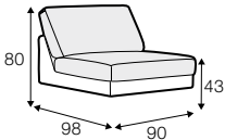
armchair wide without armrests
