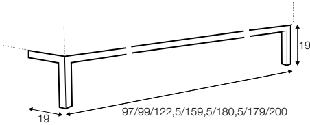
no. 146A metal chrome, painted black only front
