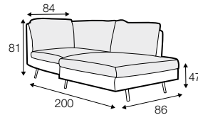
divan right / or left
