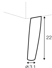
no. 210 wood front: armchair footstool
