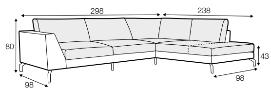
set 10 right / or left 3 seater left / or right + corner 90° + bench right / or left
