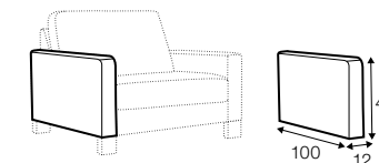
armrest 450 100x12x47 available with feet: no. 47, no. 51, no. 145B, no. 176 legs to SB H-100: no. 145B, no. 176
