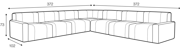
set 5 armrest + 3 x 1 seater (without ARMRESTS) + corner 90° + 3 x 1 seater (without ARMRESTS) + armrest
